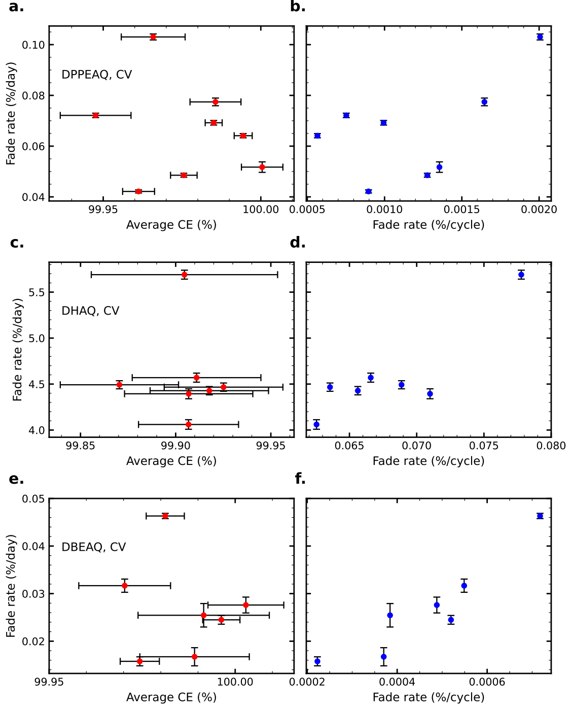
Figure S4: Instantaneous capacity fade rates of: DPPEAQ CV symmetric cells (Fig. 3) vs (a) average CE, (b) cycle-based capacity fade rates; DHAQ CV symmetric cells (Fig. 8) vs (c) average CE, (d) cycle-based capacity fade rates; DBEAQ CV symmetric cells (Fig. 9) vs (e) average CE, (f) cycle-based capacity fade rates. Error bars for instantaneous fade rates are equal to the margin of error of the regression slope at the 95% confidence level. Error bars for average CE are standard deviations. Average CE and instantaneous capacity fade rates are calculated from all cycles that occur after one day.
