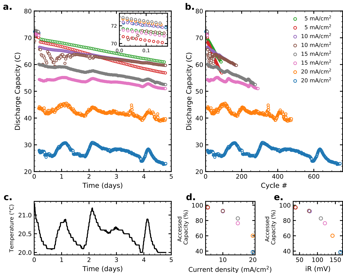
Figure 4. CC cycling of 0.1 M DHAQ pH 14 symmetric cells (4.0 ml CLS vs 6.0 ml NCLS). All cells began with 10 CV cycles ( \pm 0.2 V) to access full capacity, before switching to CC cycling. Plots of (a) temporal discharge capacity; (b) cycle-based discharge capacity; and (c) glove box temperature over time. Percent of final CV discharge half-cycle capacity accessed when switching to CC cycling, as a function of (d) applied cell current density; and (e) cell ohmic overpotential (applied current density multiplied by cell ASR).
