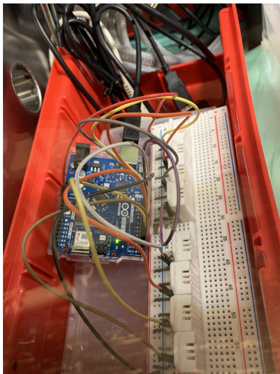
Figure S1: Arduino with temperature sensors used for glovebox temperature monitoring.
