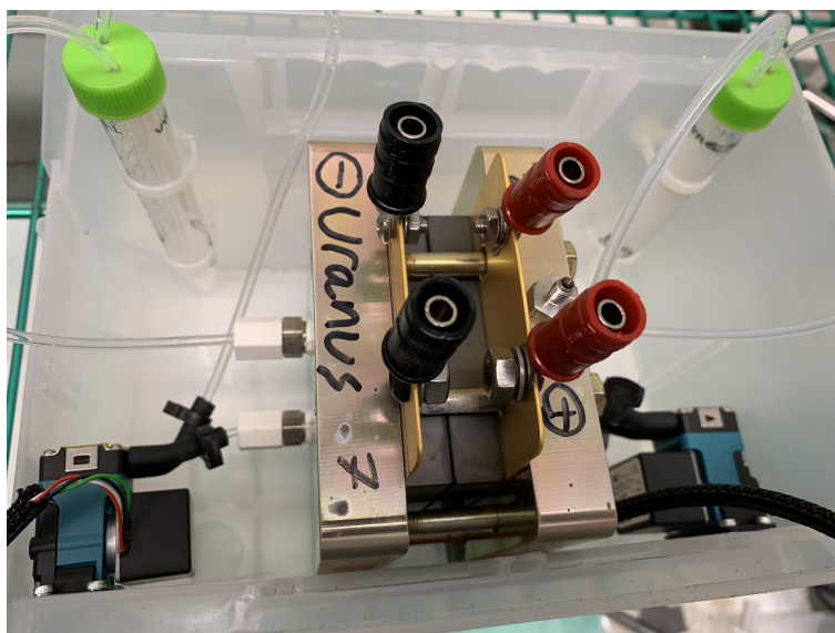
Figure S2: Modular cell, pumps, and reservoirs.
