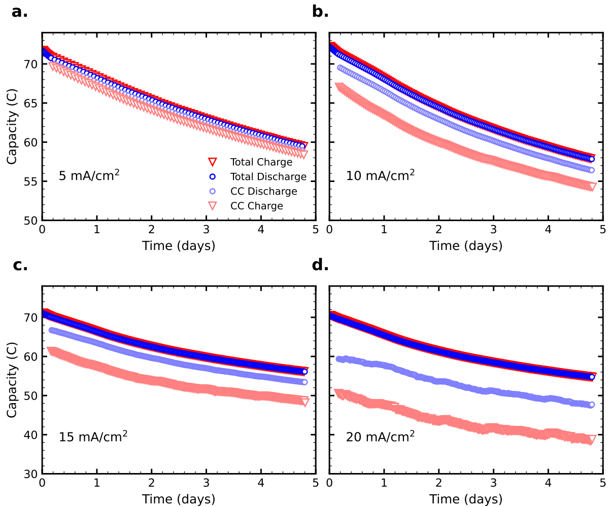
Figure S7: Capacity contribution during constant current sections of CCCV cycling protocol for representative DHAQ symmetric cells (Fig. 6) with constant current cycling performed at (a) 5 mA/cm 2 ; (b) 10 mA/cm 2 ; (c) 15 mA/cm 2 ; and (d) 20 mA/cm 2 . Note the expanded ordinate of (c)&(d) compared to (a)&(b). ‘Total charge/discharge’ represents the total capacity of the CCCV half-cycle.
