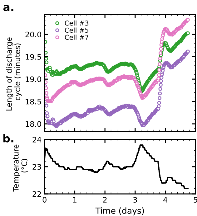
Figure S3: Select DPPEAQ symmetric cells cycled potentiostatically (from Fig. 3). (a) discharge half-cycle duration and (b) glovebox temperature, for the duration of experiment.
