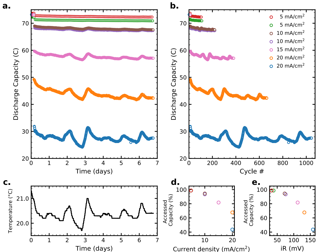
Figure 5. CC cycling of 0.1 M DBEAQ pH 14 symmetric cells (4.0 ml CLS vs 6.0 ml NCLS). All cells began with 10 CV cycles ( \pm 0.2 V) to access full capacity, before switching to CC cycling. Plots of (a) temporal discharge capacity; (b) cycle-based discharge capacity; and (c) glove box temperature over time. Percent of final CV discharge half-cycle capacity accessed when switching to CC cycling, as a function of (d) applied cell current density; and (e) cell ohmic overpotential (applied current density multiplied by cell ASR).
