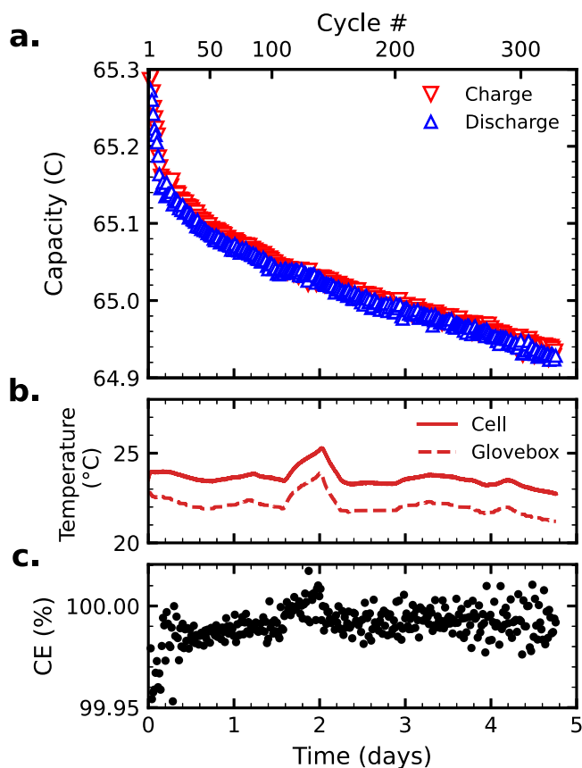
Figure 2. CV cycling ( \pm 0.2 V) of a 0.1 M DPPEAQ pH 14 symmetric cell (4.0 ml CLS vs 6.0 ml NCLS). (a) semi-log plot of temporal and cycle-based capacity; (b) cell and glove box temperatures during cycling; and (c) coulombic efficiency.
