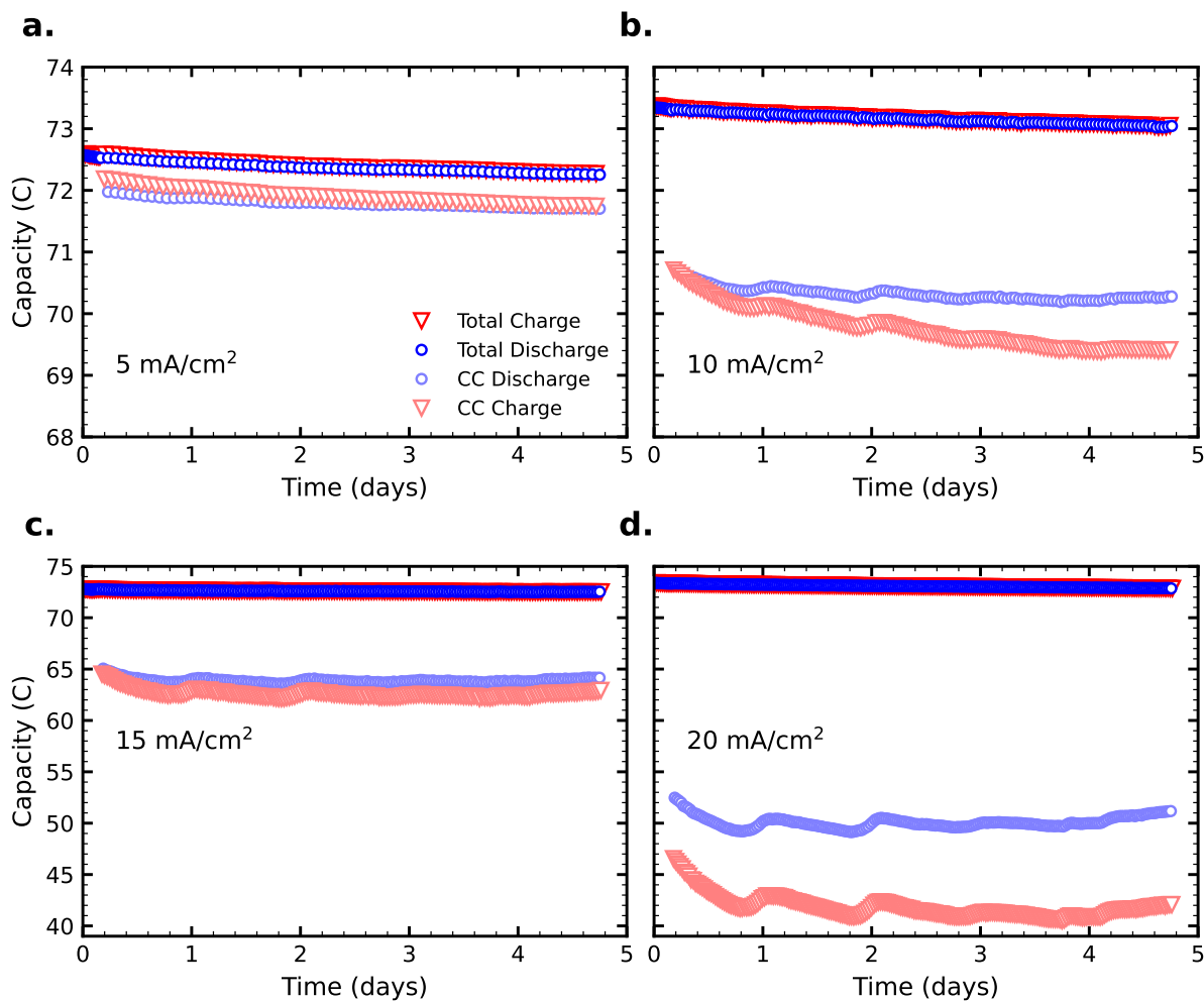
Figure S8: Capacity contribution during constant current sections of CCCV cycling protocol for representative DBEAQ symmetric cells (Fig. 7) with constant current cycling performed at (a) 5 mA/cm 2 ; (b) 10 mA/cm 2 ; (c) 15 mA/cm 2 ; and (d) 20 mA/cm 2 . Note the expanded ordinate of (c)&(d) compared to (a)&(b). ‘Total charge/discharge’ represents the total capacity of the CCCV half-cycle.
