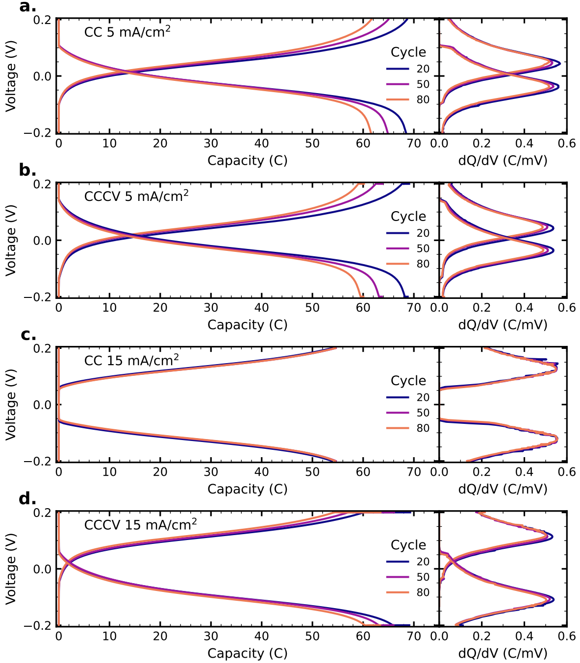
Figure S10: Voltage–charge/discharge curves (left), and differential capacity (right) evaluated as the first derivative of the voltage profiles, for DHAQ symmetric cells cycled with (a) CC 5 mA/cm 2 (cell from Fig. 4); (b) CCCV 5 mA/cm 2 (cell from Fig. 6); (c) CC 15 mA/cm 2 (cell from Fig. 4); (d) CCCV 15 mA/cm 2 (cell from Fig. 6). The cycle numbers shown do not necessarily correlate temporally across panels a–d.
