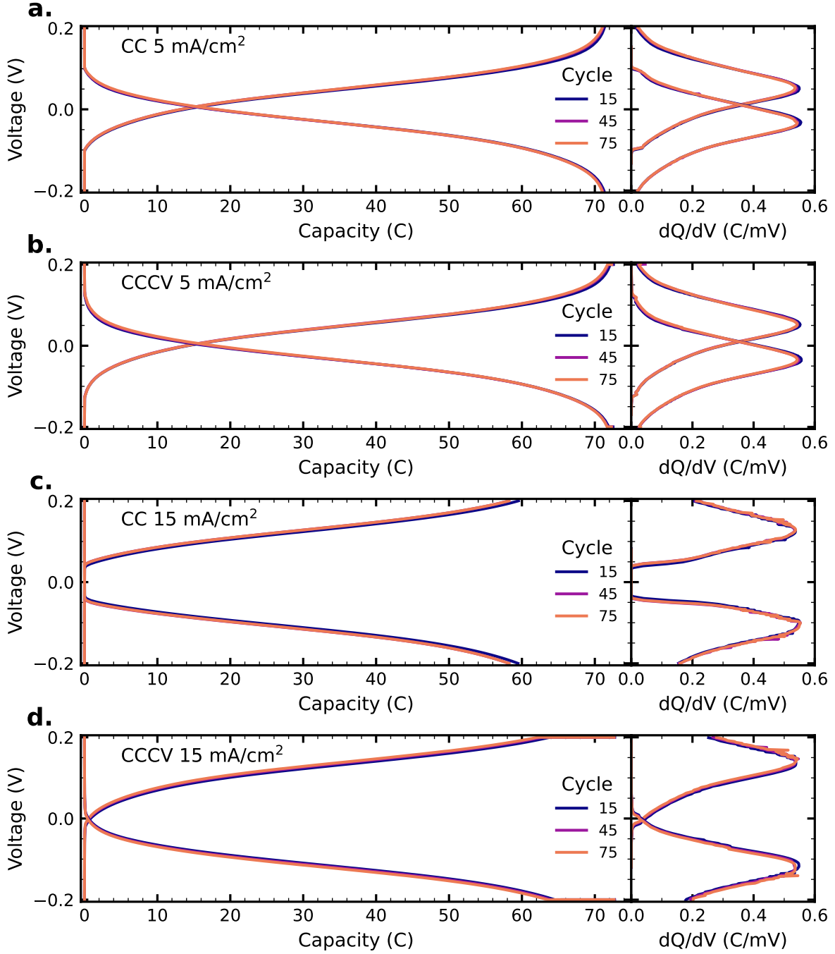
Figure S11: Voltage-charge/discharge curves (left), and differential capacity (right) evaluated as the first derivative of the voltage profiles, for DBEAQ symmetric cells cycled with (a) CC 5 mA/cm 2 (cell from Fig. 5); (b) CCCV 5 mA/cm 2 (cell from Fig. 7); (c) CC 15 mA/cm 2 (cell from Fig. 5); (d) CCCV 15 mA/cm 2 (cell from Fig. 7). The cycle numbers shown do not necessarily correlate temporally across panels a-d.
