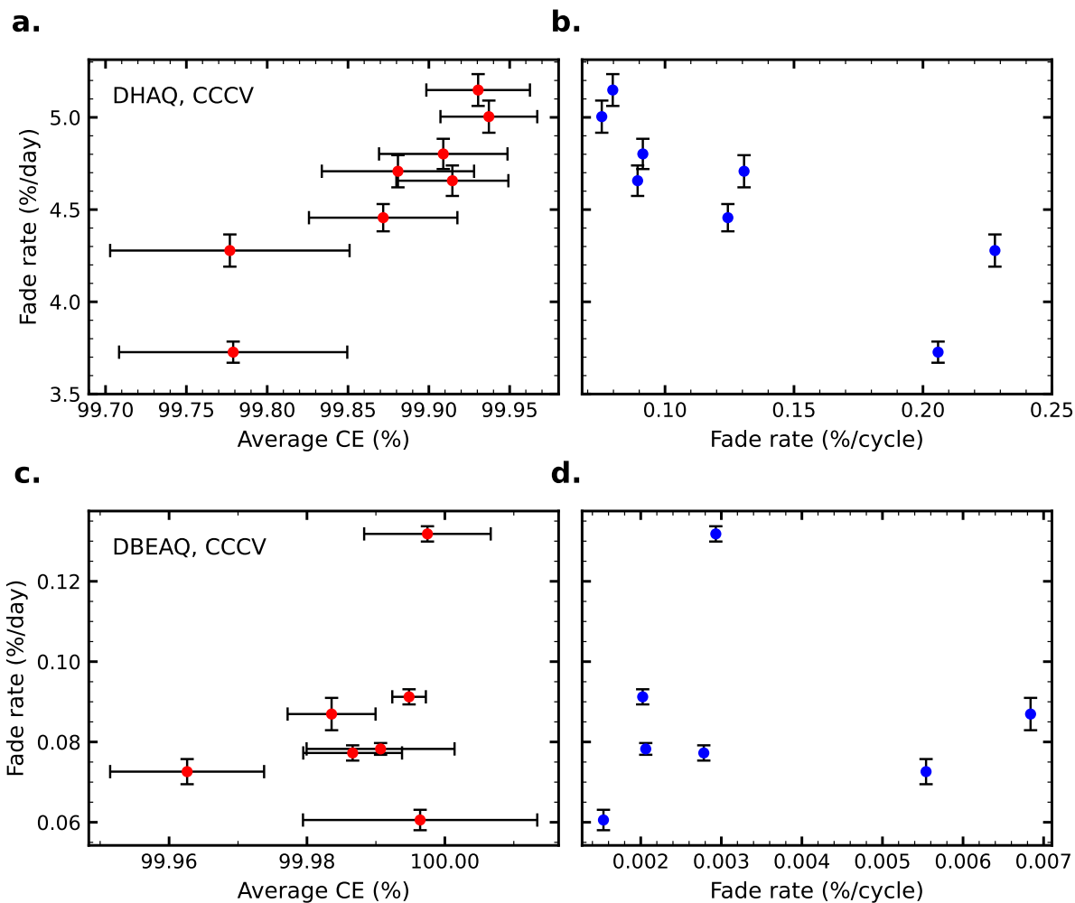
Figure S6: Instantaneous capacity fade rates of: DHAQ CCCV symmetric cells (Fig. 6) vs (a) average CE, (b) cycle-based capacity fade rates; and DBEAQ CCCV symmetric cells (Fig. 7) vs (c) average CE, (d) cycle-based capacity fade rates. Errorbars for instantaneous fade rates are equal to the margin of error of the regression slope at the 95% confidence level. Errorbars for average CE are standard deviations. Average CE and instantaneous capacity fade rates are calculated from all cycles that occur after one day.
