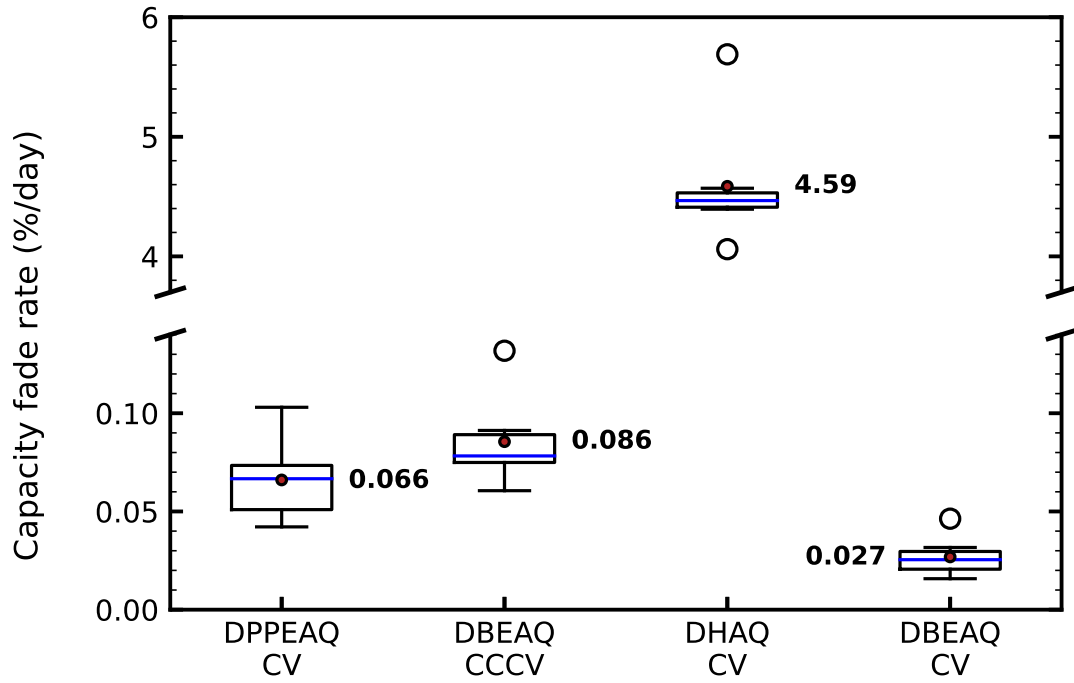
Figure S12: Variation in temporal capacity fade rates from sets of identical cells reported in the main text. Box extends from first to third quartile of the data, whiskers extend by 1.5x the inter-quartile range, white circles denote outliers, blue line is the median, and red circle denotes the (labeled) mean.
