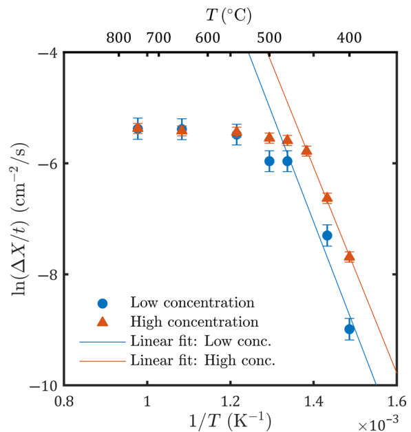
FIG. 3. Arrhenius plot of the loss of substitutionality for both low and high Au concentrations. Linear fits are obtained by total least-squares fitting using the York error-in-variable model [30] for T < 500 °C.
